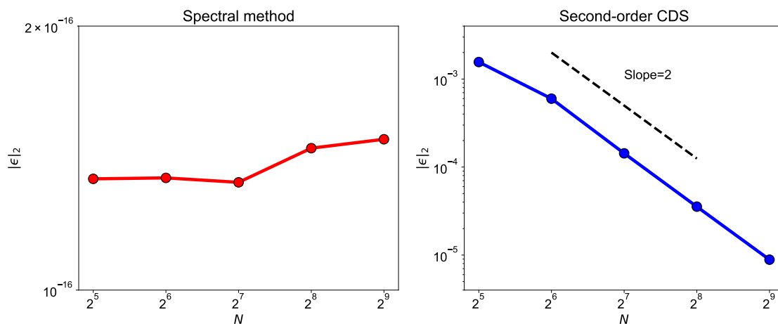
Figure 18. Order of accuracy for spectral method and second-order CDS. We calculate discretization error at five grid resolutions and change the grid size by a factor of 2 in both x and y direction. The CDS Poisson solver give second-order accuracy. Spectral method give exact solution and error is of the same order as machine zero.
