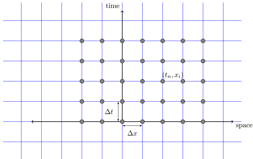
Figure 1. Finite difference grid for one-dimensional problems.
