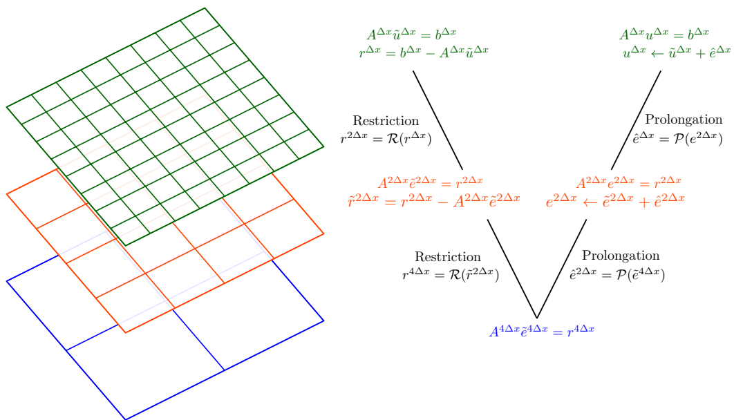
Figure 22. Illustration of multigrid V-cycle framework with three levels between fine and coarse grid. For full multigrid cycle, the coarsest mesh has 2 \times 2 grid resolution and is solved directly.
